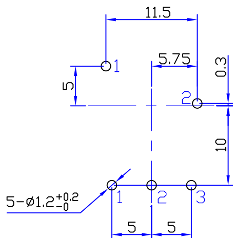
脚位安装图 Mounting hole
