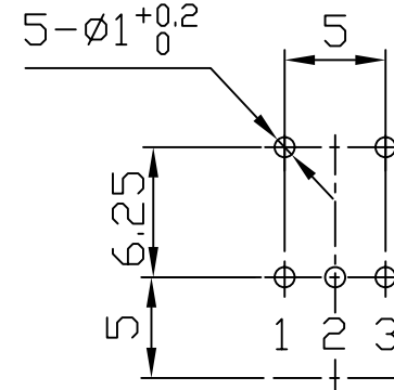
Mounting hole detail
