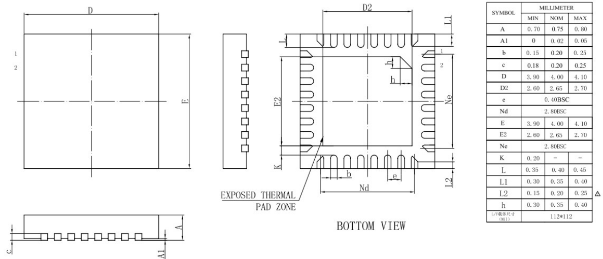
Figure 3-1. AD156B QFN32 Package
