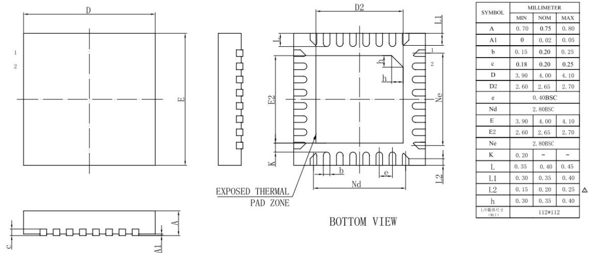
Figure 3-1. AD156A_QFN32 Package
