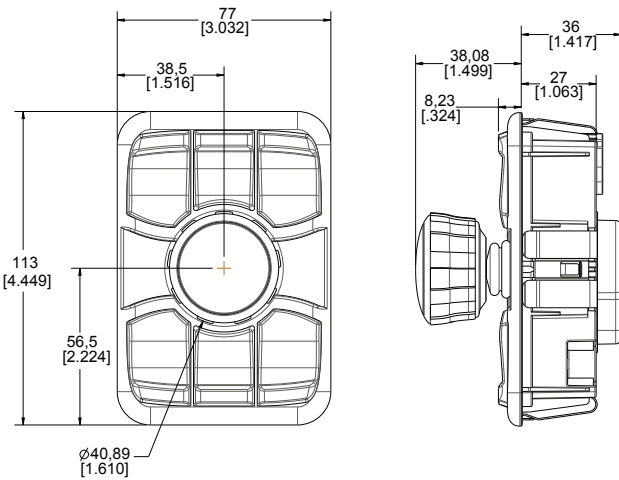
3JX2X5-G2-100X / 3JX305-G2-100X PROPORTIONAL JOYSTICK / DUAL PROPORTIONAL OUTPUT VERSION
