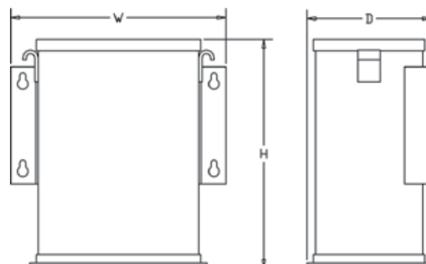
Design Style 2 - Type 4, Type 4X, Type 12
