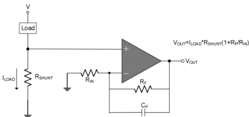
Figure11.Low-SideCurrentMonitor
