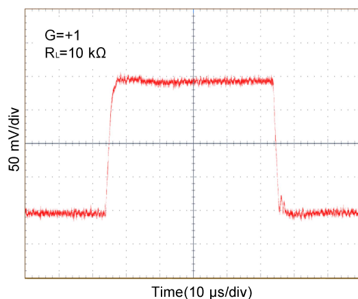
Figure 5 SMALL-SIGNAL STEP RESPONSE at +2.7V
