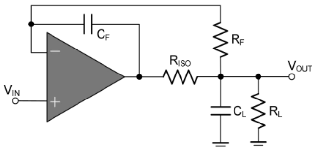
Figure10.IndirectlyDrivingCapacitiveLoadwithDCAccuracy
