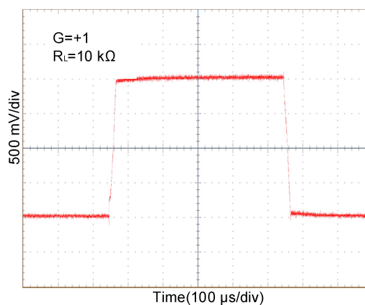
Figure 3 LARGE-SIGNAL STEP RESPONSE at +2.7V
