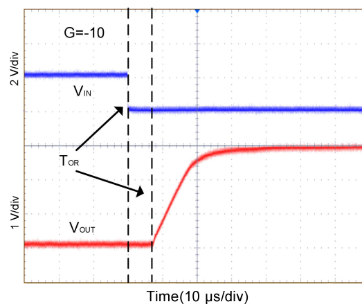
Figure 7 NEGATIVE OVERLOAD RECOVERY
