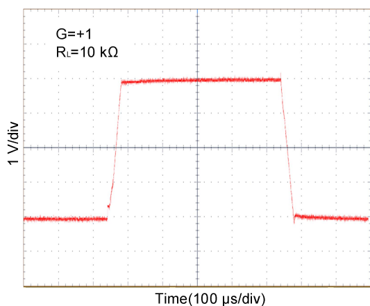
Figure 2 LARGE-SIGNAL STEP RESPONSE at +5V
