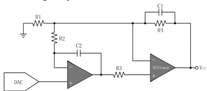
Figure13.ProgrammablePowerSupply
