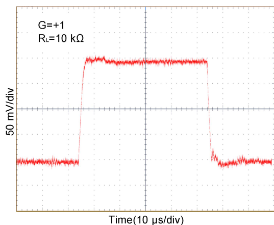
Figure 4 SMALL-SIGNAL STEP RESPONSE at +5V
