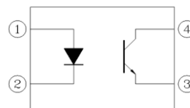
Pin Configuration
