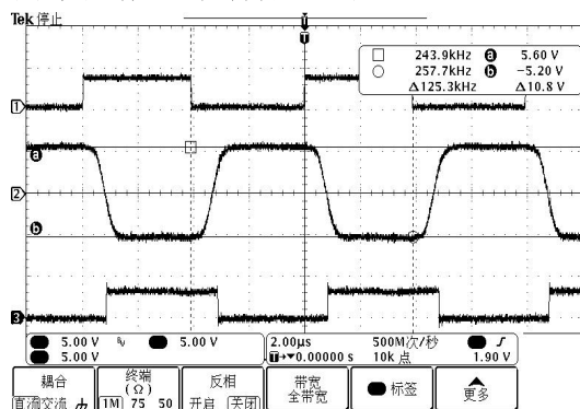
图2. WS3222E TIN to TOut to ROut (loopbackto Rx with 1000pF load) at 250kbps waveform
