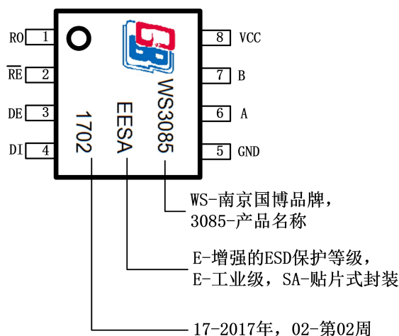
WS3085 引脚图—8-pin SOP (Top View)
