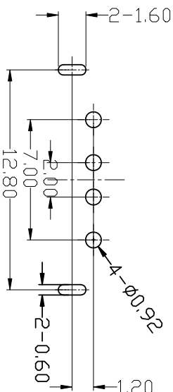
FRONT EDGE OF CONNECTOR PCB LAYOUT (T=1.60mm)
