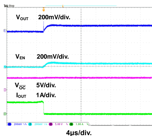
Figure 14. Output Load Insert Hot Plug-Off with 4\Omega (1.25A)
