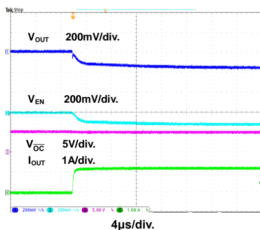
Figure 13. Output Load Insert Hot Plug-In with 4\Omega (1.25A)
