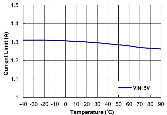
Figure 19. Current Limit vs. Temperature
