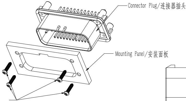
Four Mounting Screws/4个安装螺丝 Torque/扭矩0.6N.m-0.8N.m
