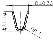
SECTION:H-H
