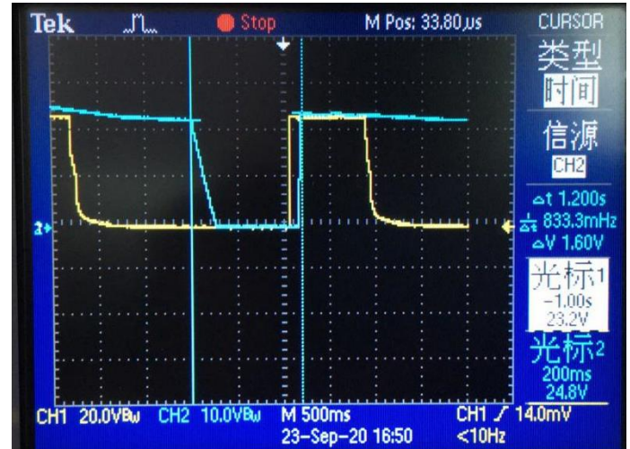
Output response & load (24V / 1.5A)
