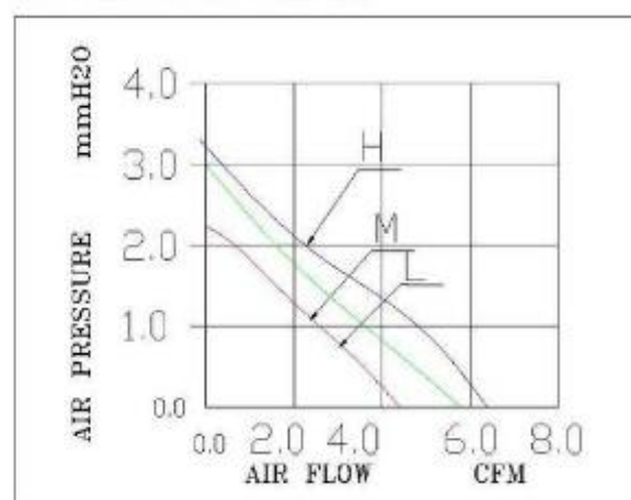
Air Floe vs Air Pressure
