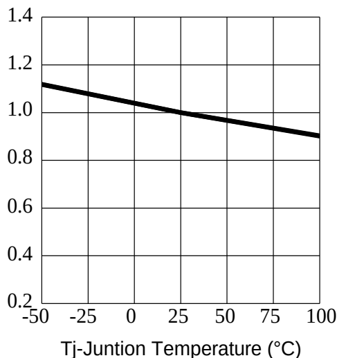
Fig. 3 - Relative Luminous Intensity vs. Junction Temperature
