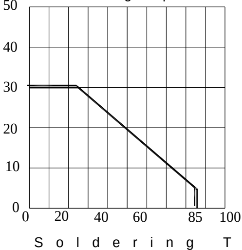
Fig. 5 - Max. Driving Current vs. Soldering Temperature
