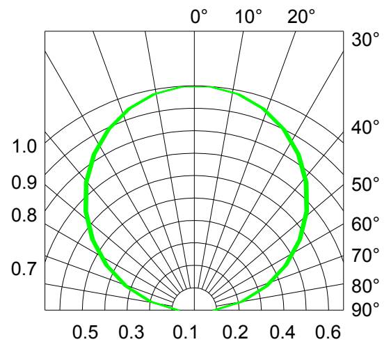
Fig.6-Radiation Diagram Ta=25°C
