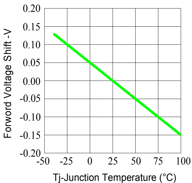
Fig.1-Forward Voltage Shift vs. Junction Temperature
