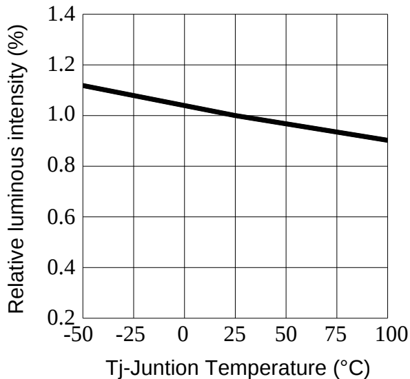
Fig.3-Relative Luminous Intensity vs.Junition Temperature
