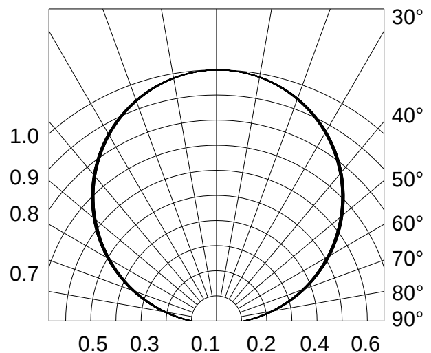
Fig.6-Radiation Diagram T_a=25^{\circ}\text{C} 0° 10° 20°
