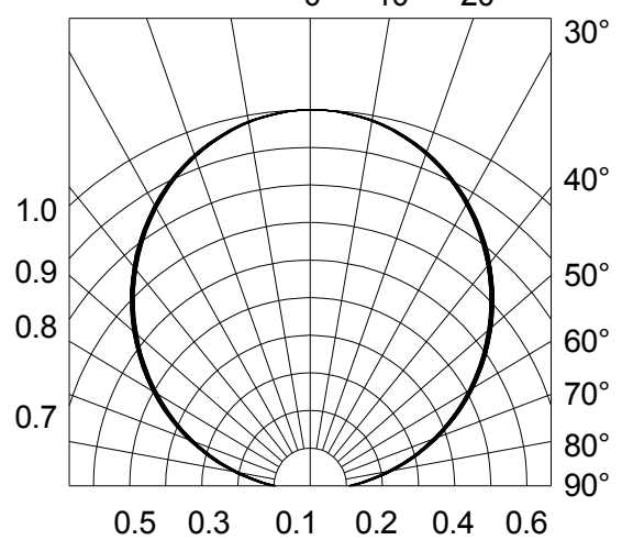
Fig.6-Radiation Diagram T_a=25^{\circ}\text{C}
