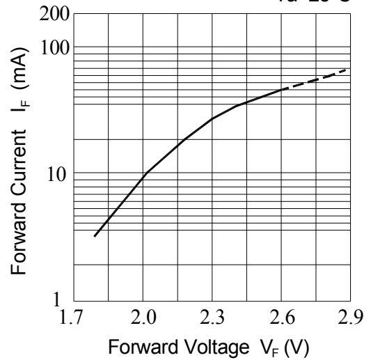
Fig.4-Forward Current vs. Forward Voltage T_a=25^{\circ}\text{C}
