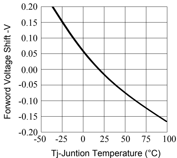
Fig.1-Forward Voltage Shift vs. Juntion Temperature
