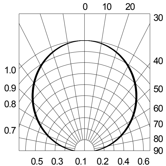
Fig.6-Radiation Diagram T_a=25^\circ\text{C}
