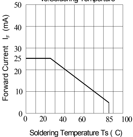
Fig.5-Max.Driving Forward Current vs.Soldering Temperture
