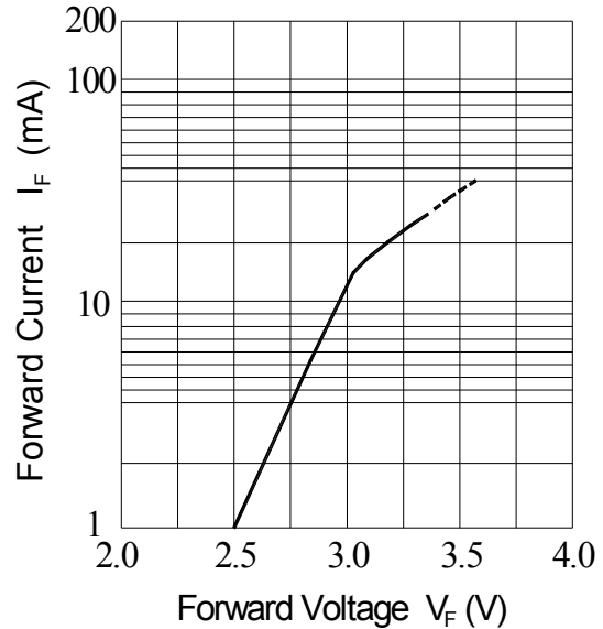
Fig.4-Forward Current vs. Forward Voltage T_a=25^\circ\text{C}
