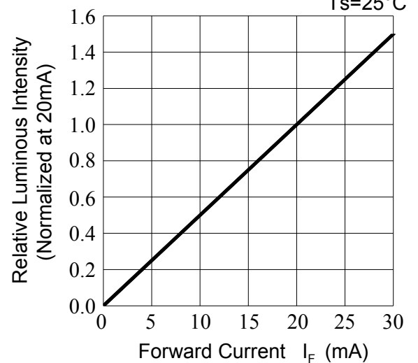
Fig.2-Relative Luminous Intensity vs. Forward Current Ts=25°C
