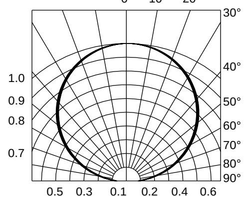
Fig.6-Radiation Diagram Ta=25°C
