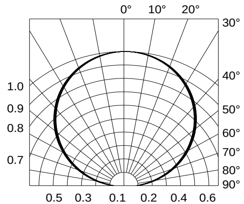
Fig.6-Radiation Diagram T_a = 25^\circ\text{C}
