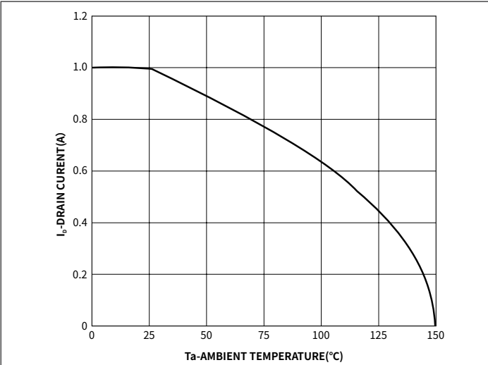
Fig.7 Drain Current vs. Temperature
