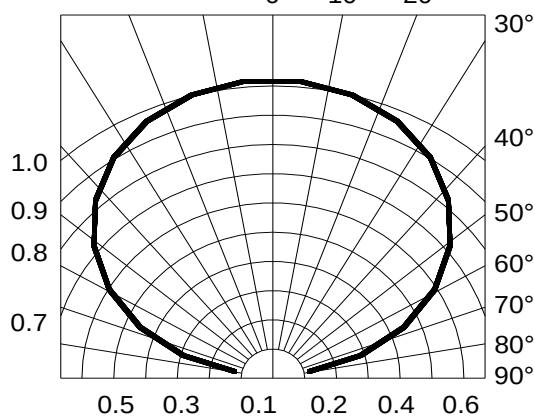
Fig.6-Radiation Diagram
