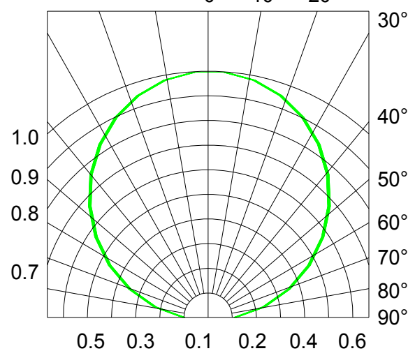
Fig.6-Radiation Diagram T_a=25^\circ\text{C}
