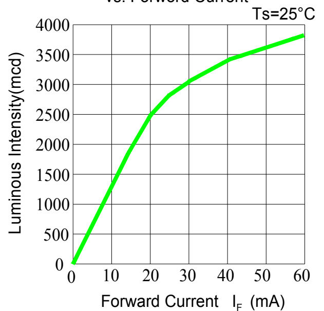
Fig.2- Luminous Intensity vs. Forward Current
