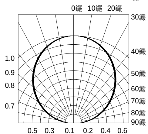
Fig.6-Radiation Diagram Ta=25°C
