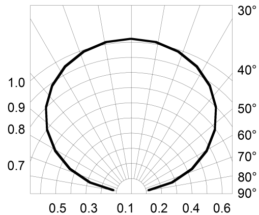
Fig.6-Radiation Diagram T_a=25^\circ\text{C}
