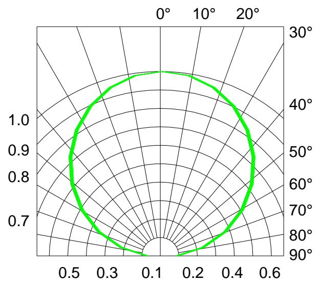
Fig.6-Radiation Diagram T_a=25^\circ\text{C}
