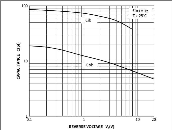
Fig.6 Cob/Cib- V_{ce}
