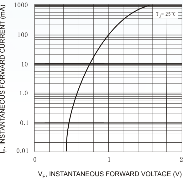
Fig. 1 Forward Characteristics
