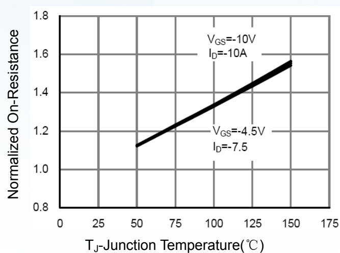
Figure 8 Drain-Source On-Resistance
