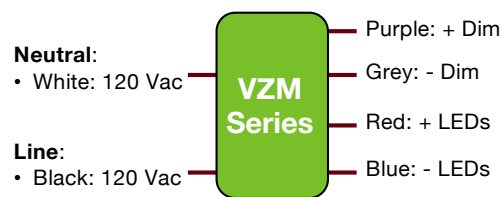
Wiring Diagram
