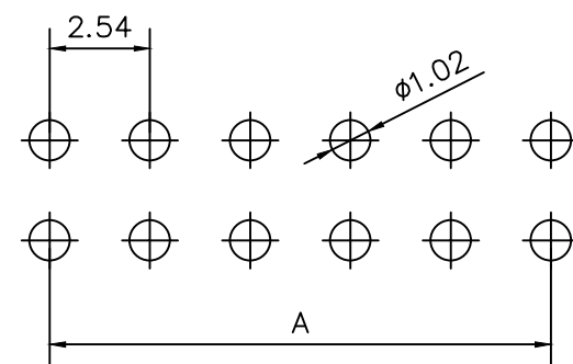
RECOMMEND P.C.B LAYOUT PCB TOLERANCE: ±0.05 (TOP VIEW)
