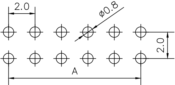
RECOMMEND P. C. B LAYOUT PCB TOLERANCE:±0.05 (TOP VIEW)
