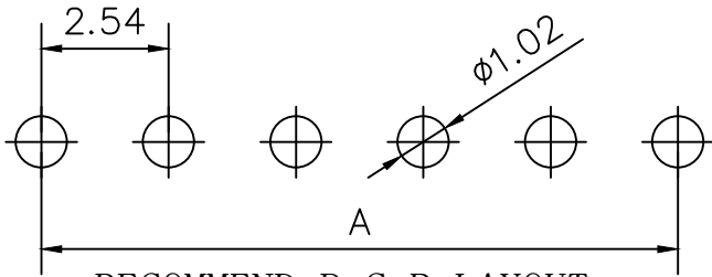
RECOMMEND P. C. B LAYOUT PCB TOLERANCE:±0.05 (TOP VIEW)
