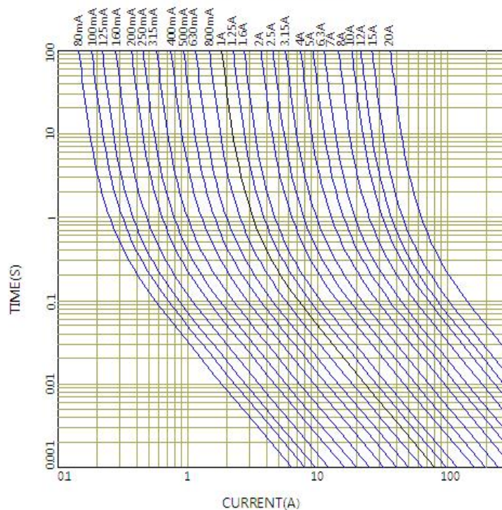
I-T CURVE
