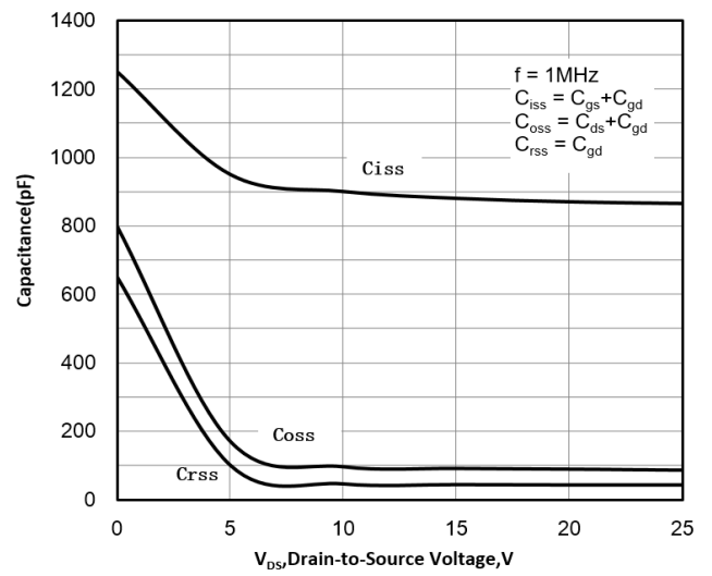
Figure 8 Capacitance Characteristics
