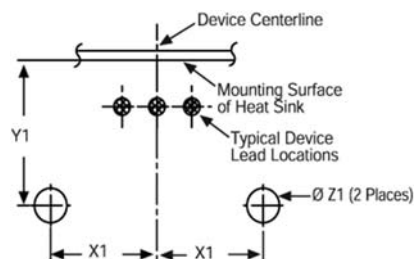
Mounting Details:
