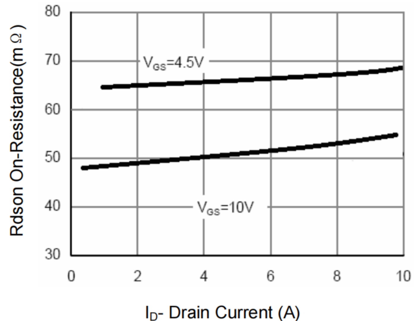
Figure 6 Drain-Source On-Resistance
