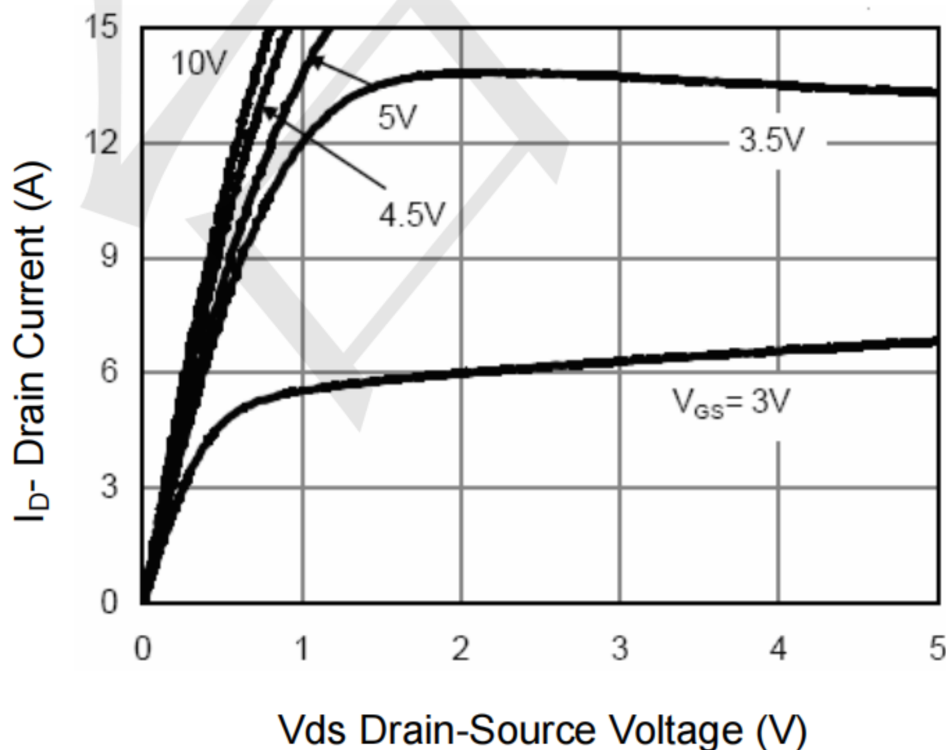
Figure 5 Output Characteristics
