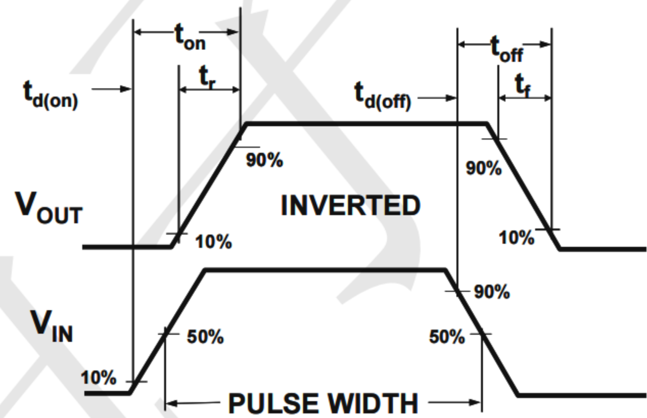
Figure 2: Switching Waveforms
