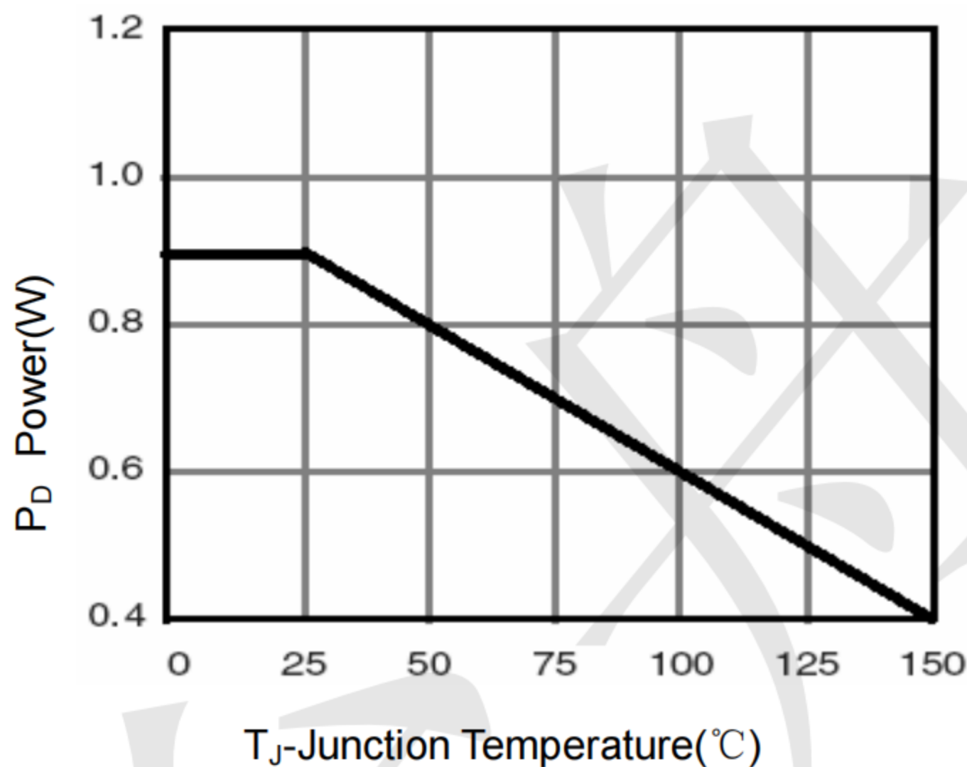
Figure 3 Power Dissipation
