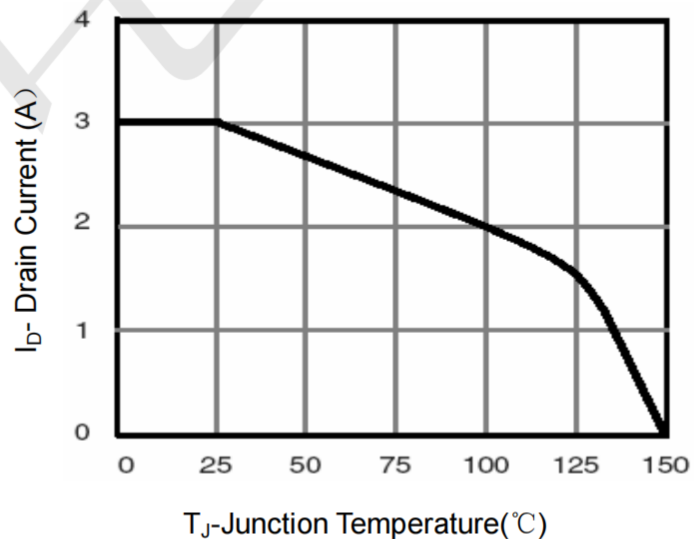
Figure 4 Drain Current
