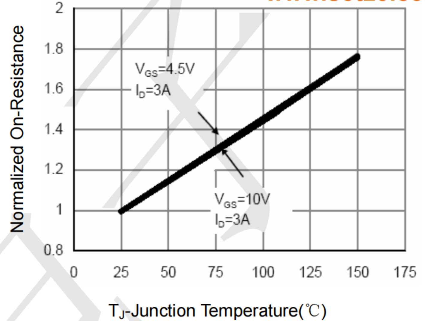
Figure 8 Drain-Source On-Resistance
