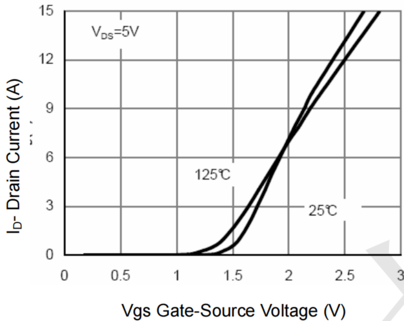
Figure 7 Transfer Characteristics
