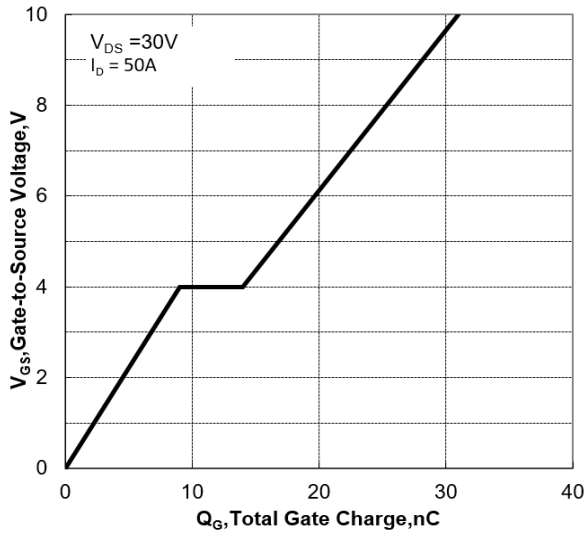
Figure 7 Gate-Charge Characteristics
