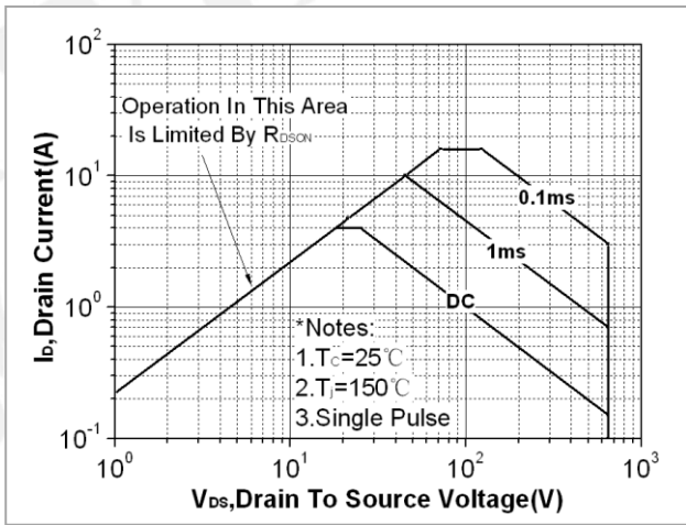
Fig. 10. Maximum safe operating area (TO-251N & TO-251S & TO-251M & TO-251U & TO-252 & TO-251MQ)
