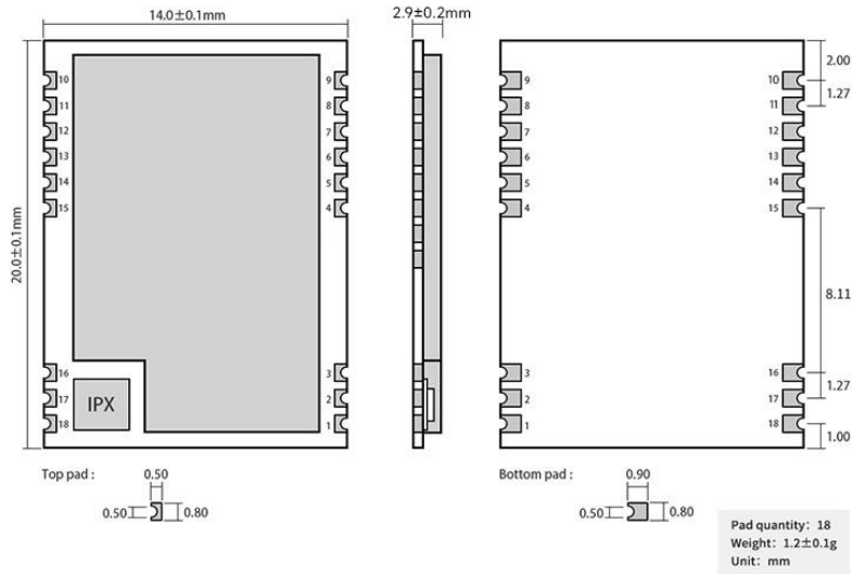
Image 3-1 Mechanical Dimensions and Pin Definition
