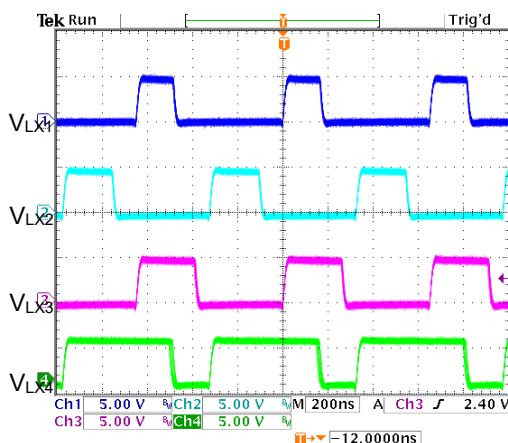
Each Channel 1A Loading LX Waveform
