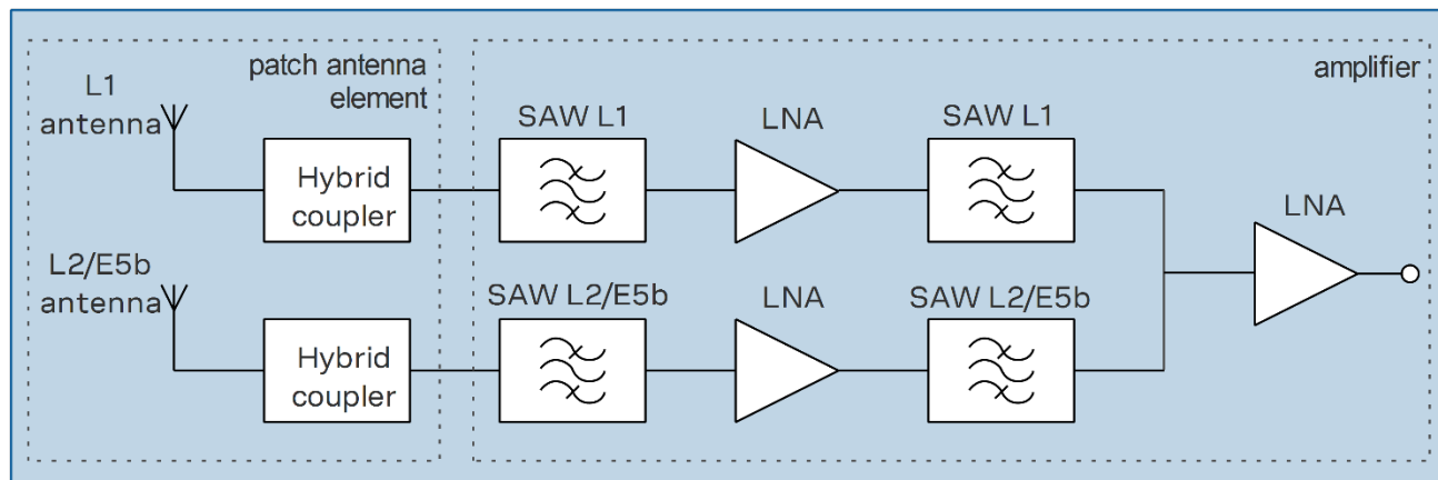
Figure 2: Simplified ANN-MB series block diagram
