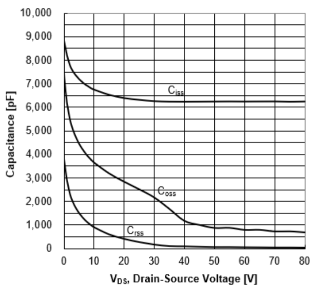
Figure 12. Capacitance Characteristics
