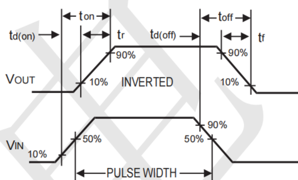
Figure 10. Switching Waveforms
