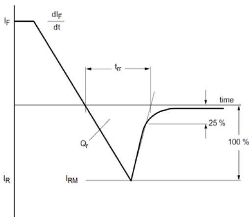
Fig. 5 Reverse recovery definitions; ramp recovery
