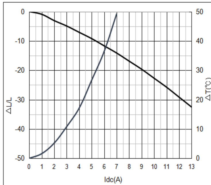
3R3 DC Bias & Temperature Characteristics
