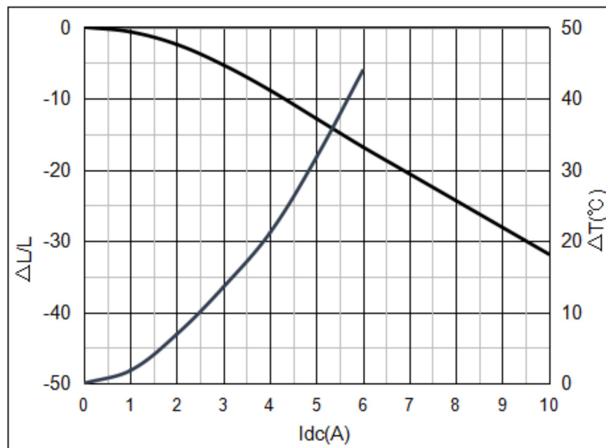
4R7 DC Bias & Temperature Characteristics
