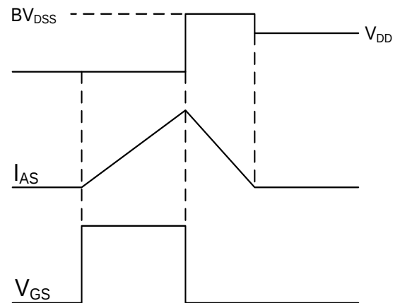
Fig.12 EAS Waveform
